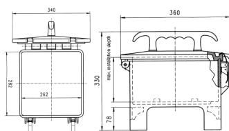
Drawing 5 MB 43 Dim. in mm
