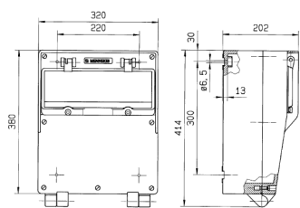
Drawing 5 MB 41 Dim. in mm
