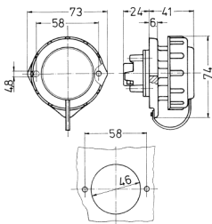
Drawing 1 MB 301 Dim. in mm
