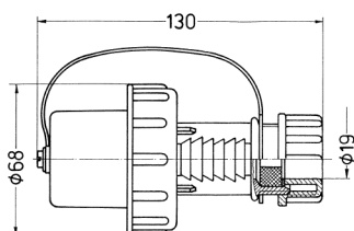
Drawing 2 MB 163 Dim. in mm
