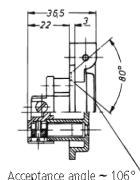
Drawing 1 MB 421 Dim. in mm
